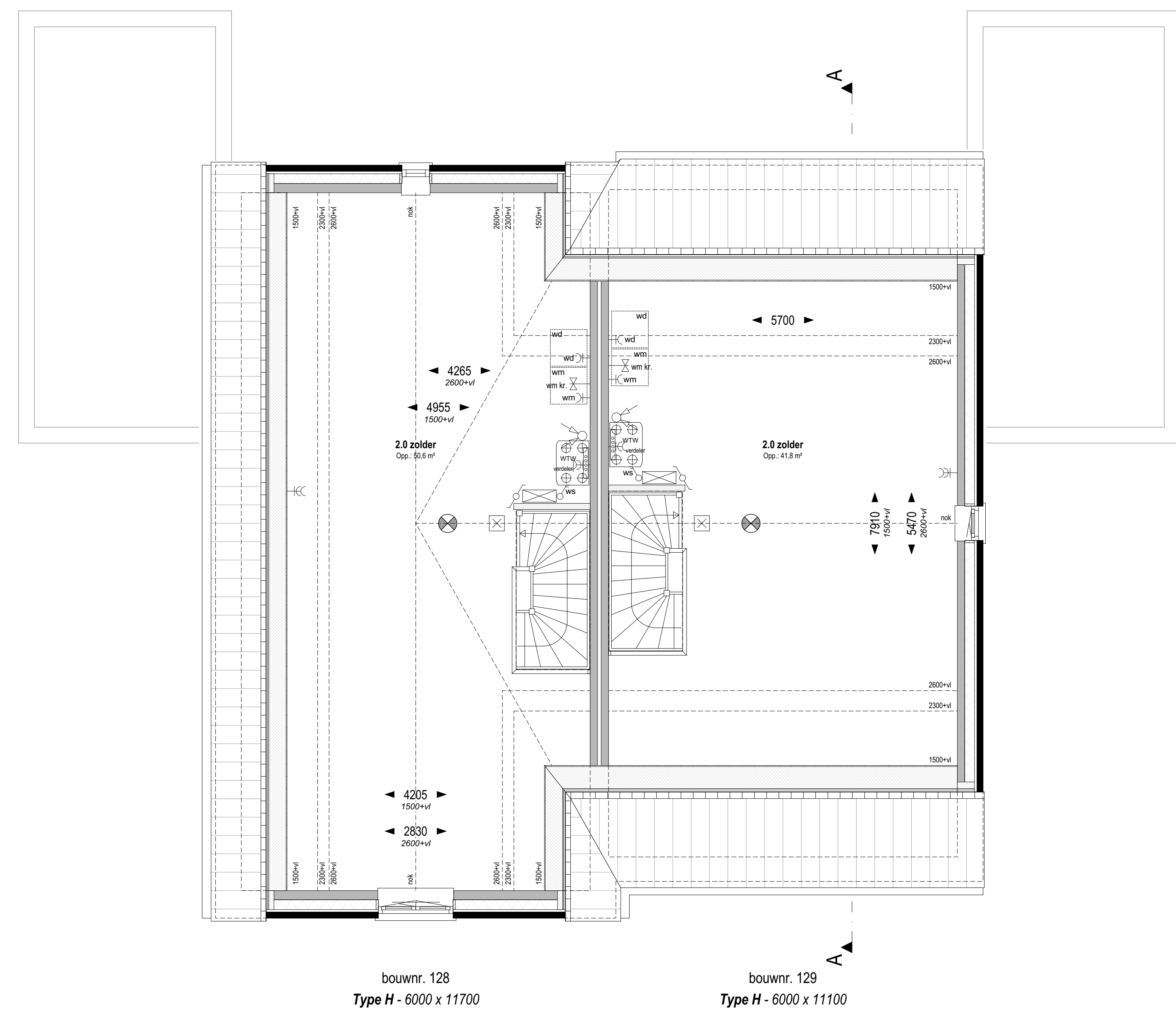
Zolder +5840 (1:50)
