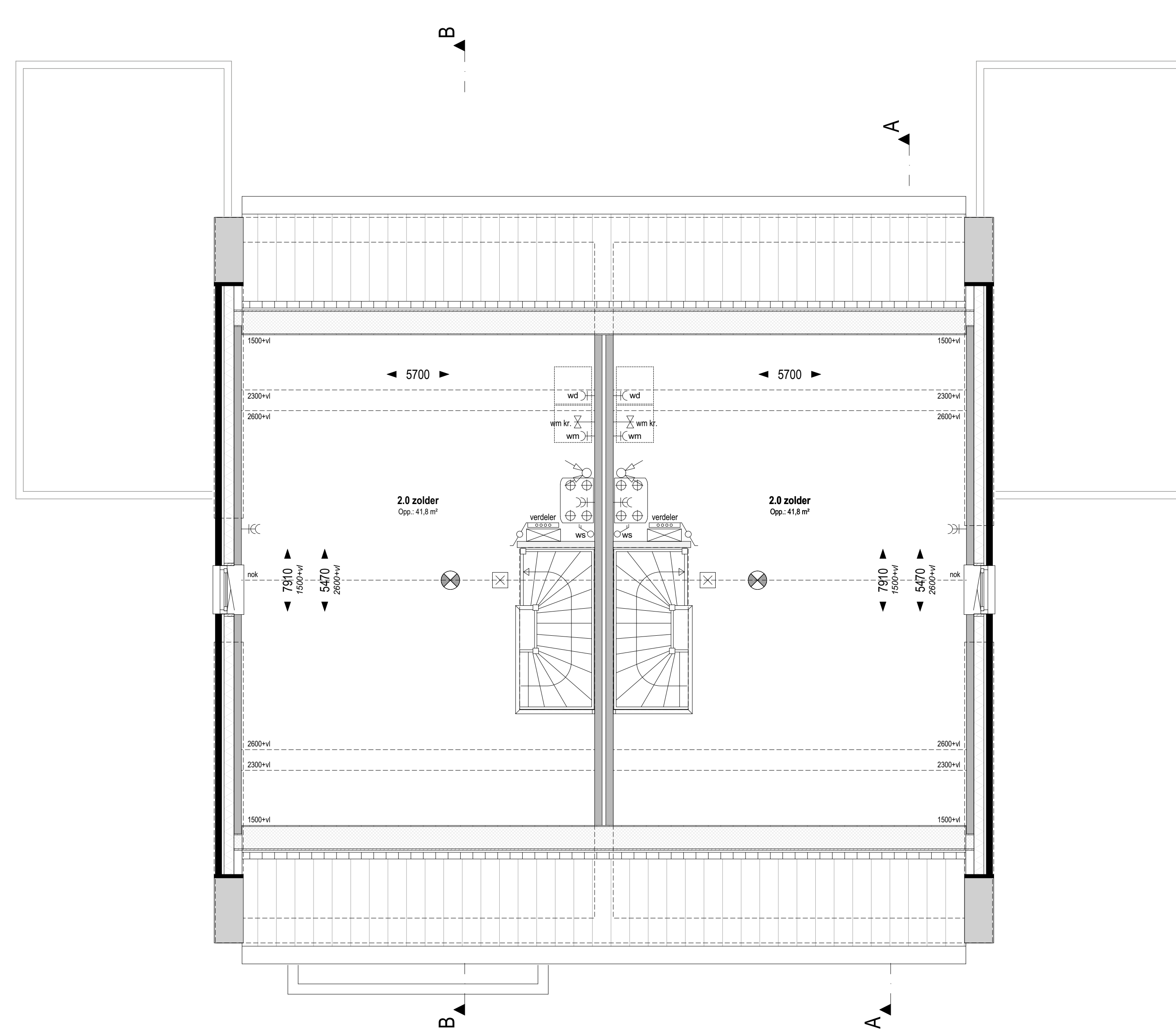
Zolder +5840 (1:50)
