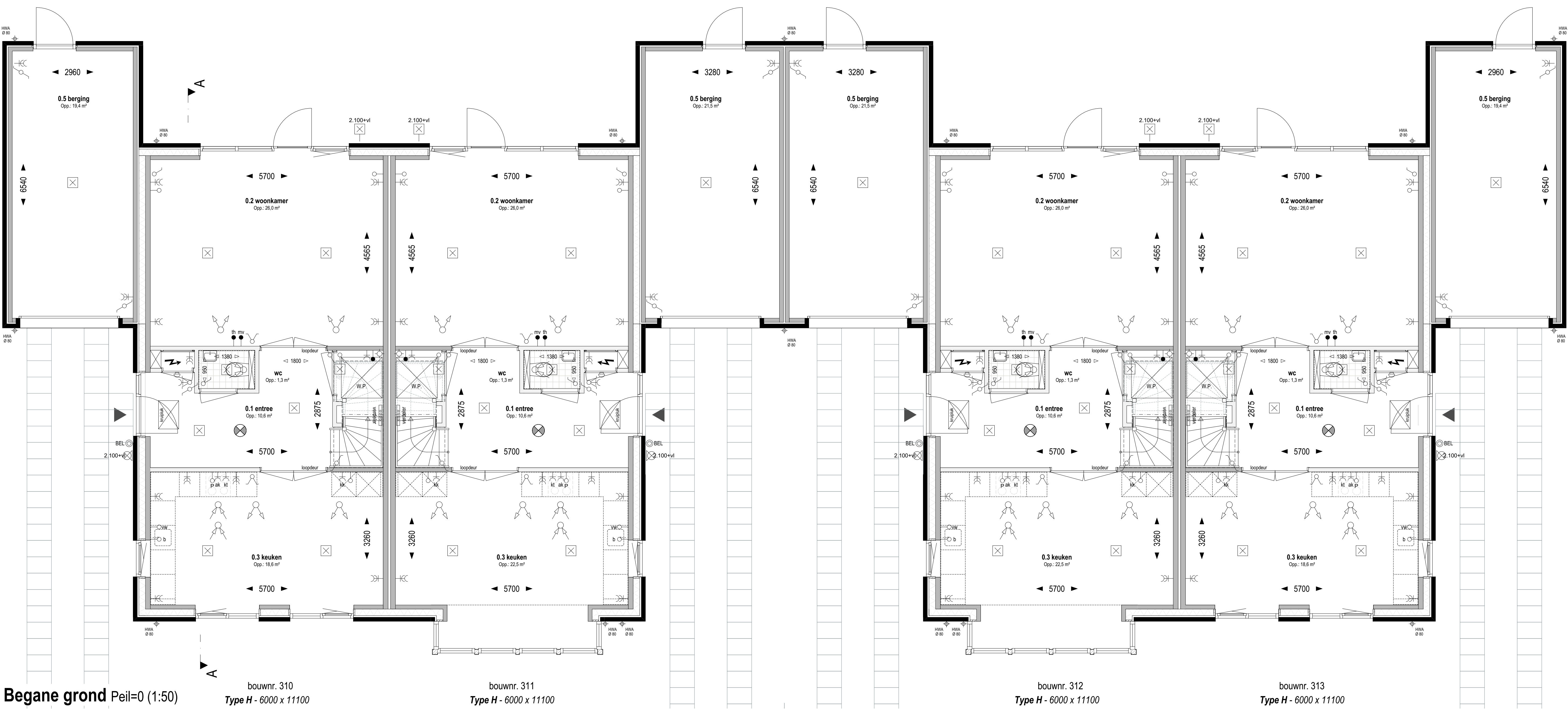
Begane grond Peil=0 (1:50)
